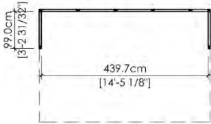
■ 3M X 4.5M INLINE [inline 10' x 15']
