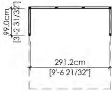
■ 3M X 4.5M INLINE [inline 10' x 15']
