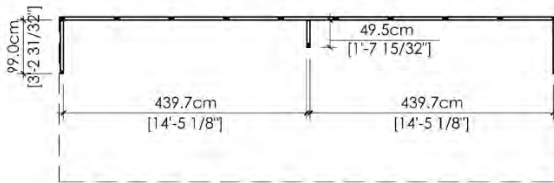
■ 3M X 9M INLINE - OPTION 1 [inline 10' x 30']
