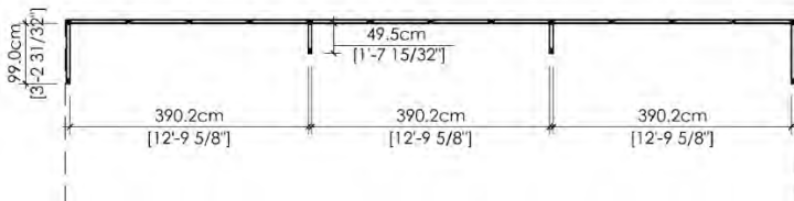
■ 3M X 12M INLINE - OPTION 1 [inline 10' x 40']
