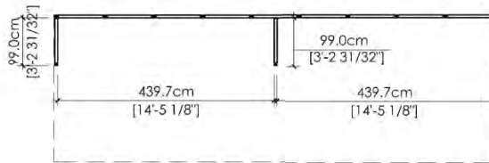
■ 3M X 9M INLINE - OPTION 2 [inline 10' x 30']
